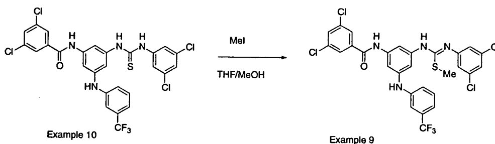
Scheme II-C
